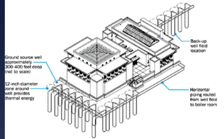
DIAGRAM OF GEOTHERMAL HVAC SYSTEM
