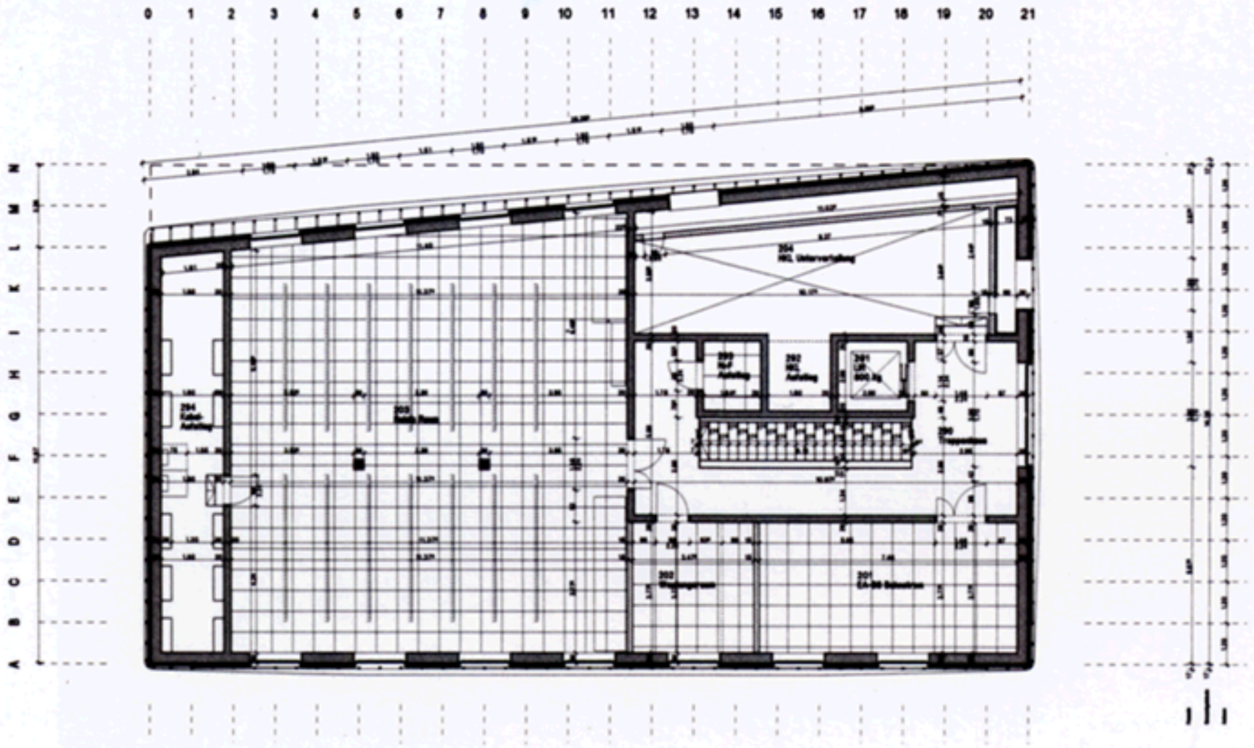
Planta segunda / Second floor plan
