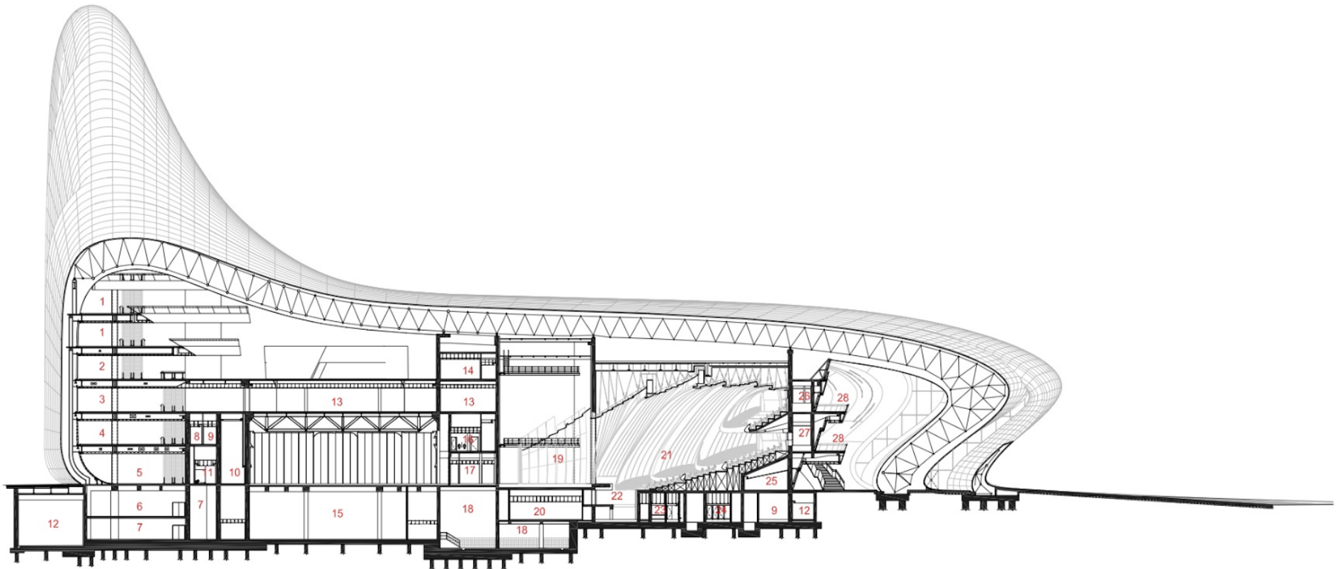
Section A-A Heydar Aliyev Centre
